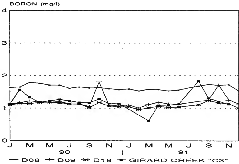
Figure 4.4 Boron for Selected Discharge Points, 1990 and 1991.
